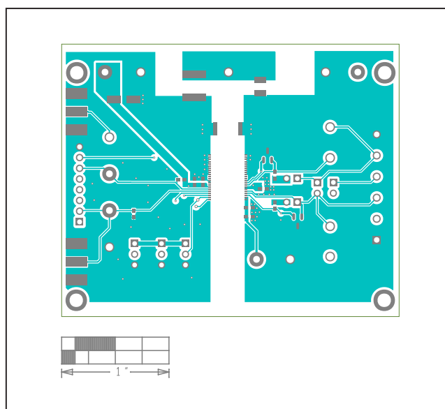
MAXM22510/MAXM22511 EV Kit—Top
