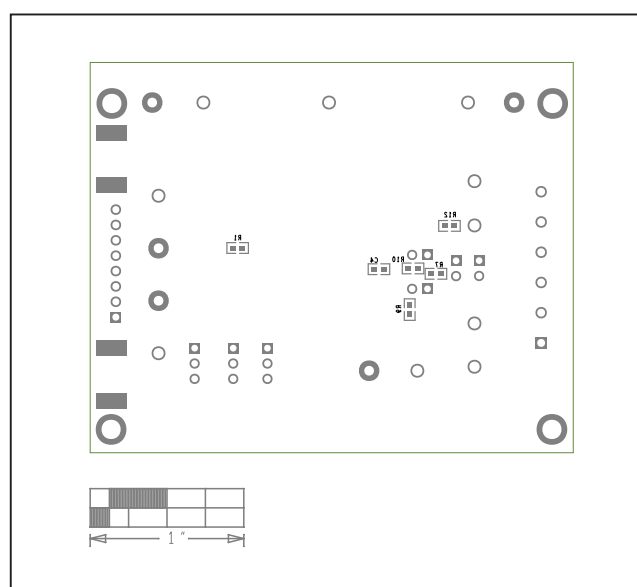
MAXM22510/MAXM22511 EV Kit—Bottom Silkscreen
