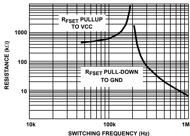
FIGURE 1. R_{FSET} RESISTANCE vs FREQUENCY
