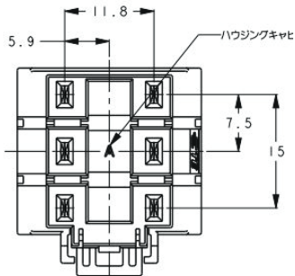
Receptacle Assembly
