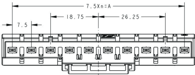
Receptacle Assembly
