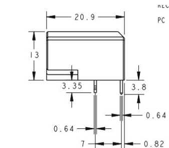
Board Mount Header Assembly
