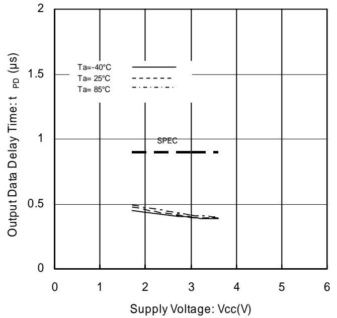
Figure 21. Output Data Delay Time vs Supply Voltage (HIGH)
