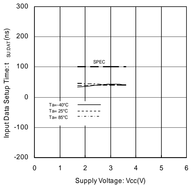
Figure 19. Input Data Setup Time vs Supply Voltage
