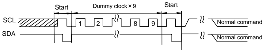
Figure 34.-(b) The case of START + dummy clockx9 + START + command input
