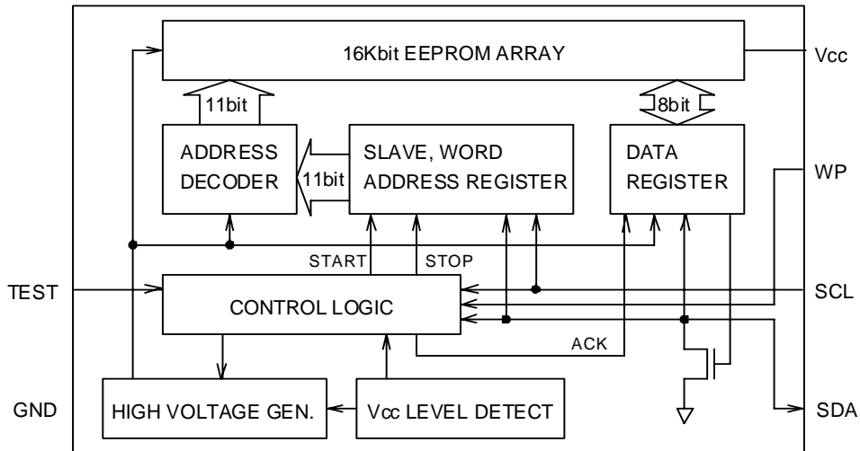
Figure 2. Block Diagram
