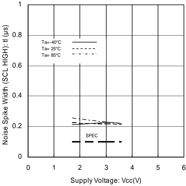
Figure 24. Noise Spike Width vs Supply Voltage (SCL H)
