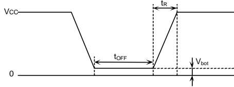
Figure 45. Rise Waveform Diagram
