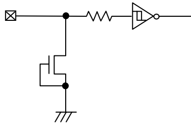
Figure 43. Input Pin Circuit Diagram
