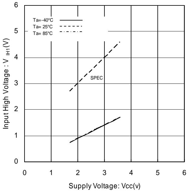
Figure 4. Input High Voltage1 vs Supply Voltage
