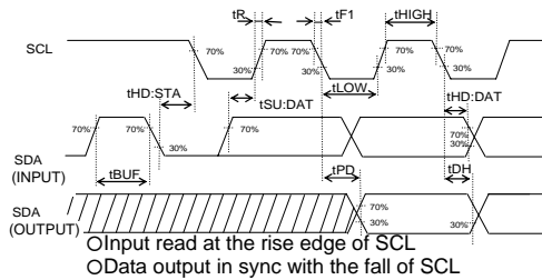
Figure 1.-(a). Serial Input / Output Timing
