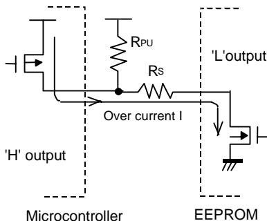
Figure 42. I/O circuit diagram
