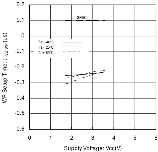
Figure 26. WP Setup Time vs Supply Voltage
