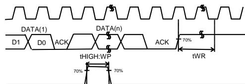
Figure 1.-(e). WP Timing at Write Cancel
