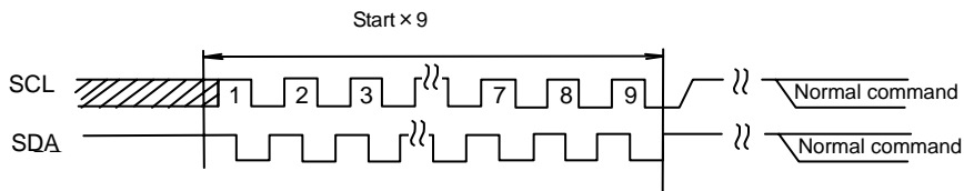
Figure 34.-(c) STARTx9 + command input
