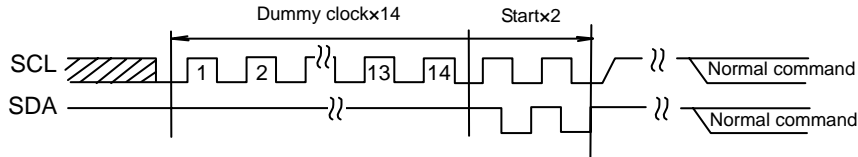
Figure 34.-(a) The case of dummy clockx14 + START+START+ command input
