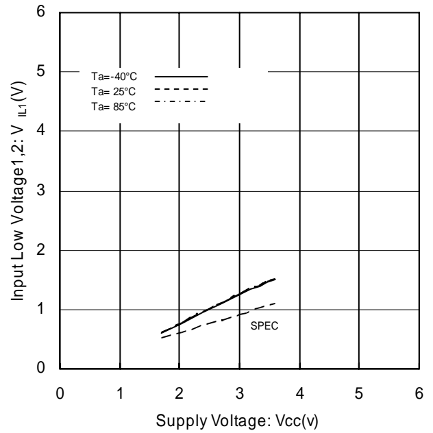
Figure 5. Input Low Voltage1 vs Supply Voltage
