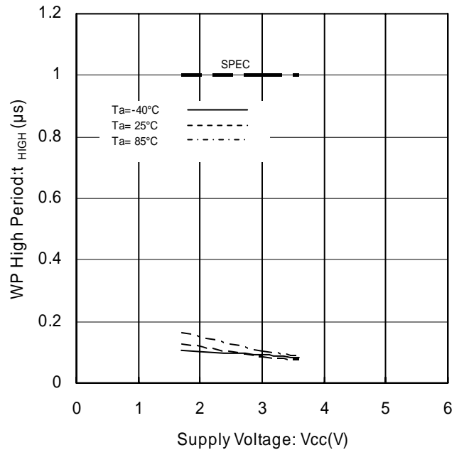
Figure 27. WP High Period vs Supply Voltage
