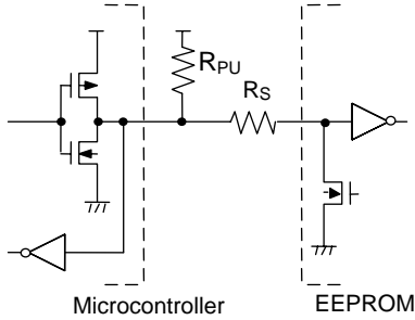
Figure 39. I/O Circuit Diagram
