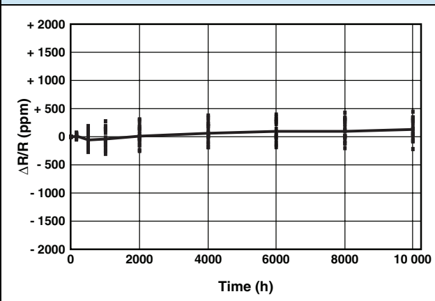
FIGURE 3 - 1240W 10 kΩ LOAD LIFE, 20 UNITS, 10 000 h at 0.25 W, + 85 °C (Wiper at CW)
