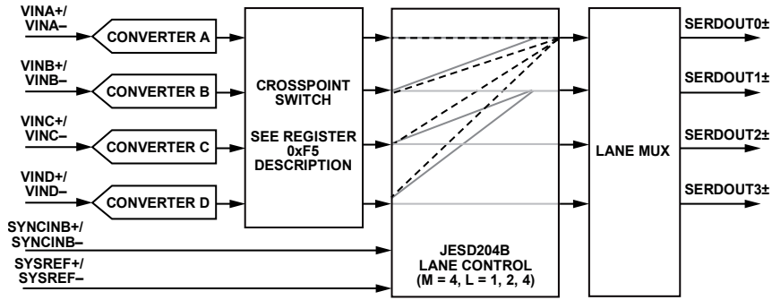
Figure 68. AD9656 Transmit Link Simplified Conceptual Block Diagram
