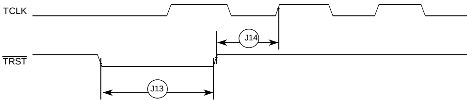
Figure 26. TRST Timing
