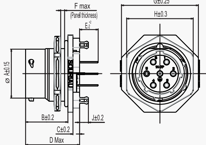
MATING FACE
