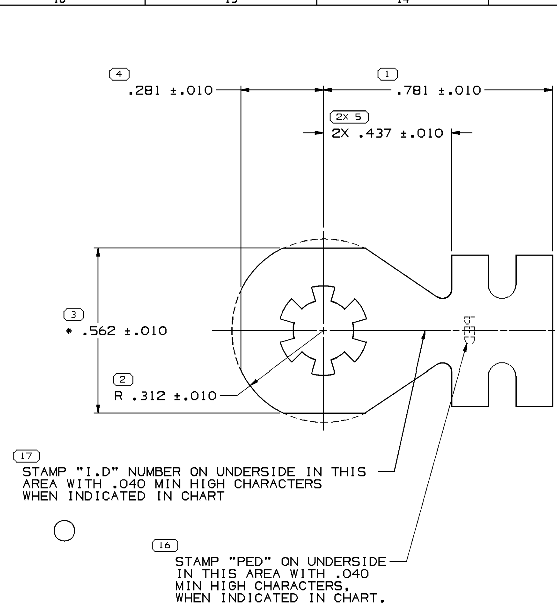
TYPE 101 BLANK VIEW (APPROX)
