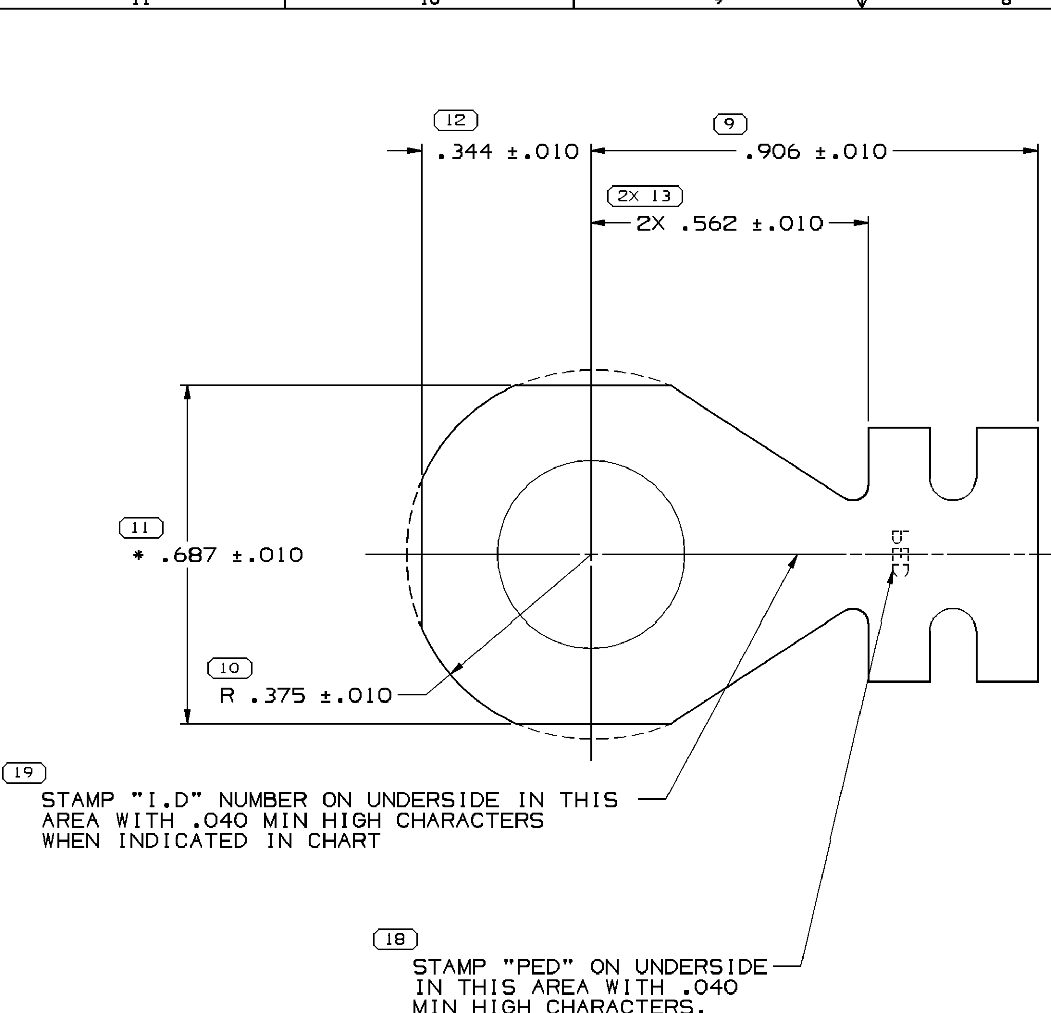
TYPE 102 BLANK VIEW (APPROX)
