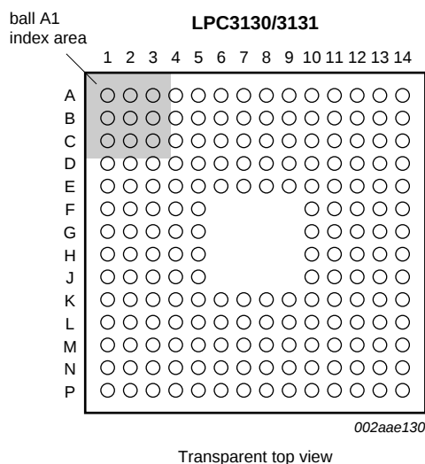
Fig 2. LPC3130/3131 pinning TFBGA180 package
