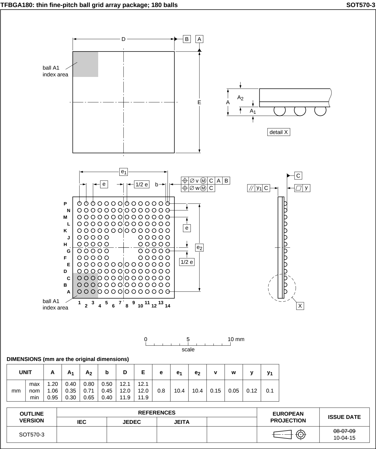
Fig 24. LPC3130/3131 TFBGA180 package outline
