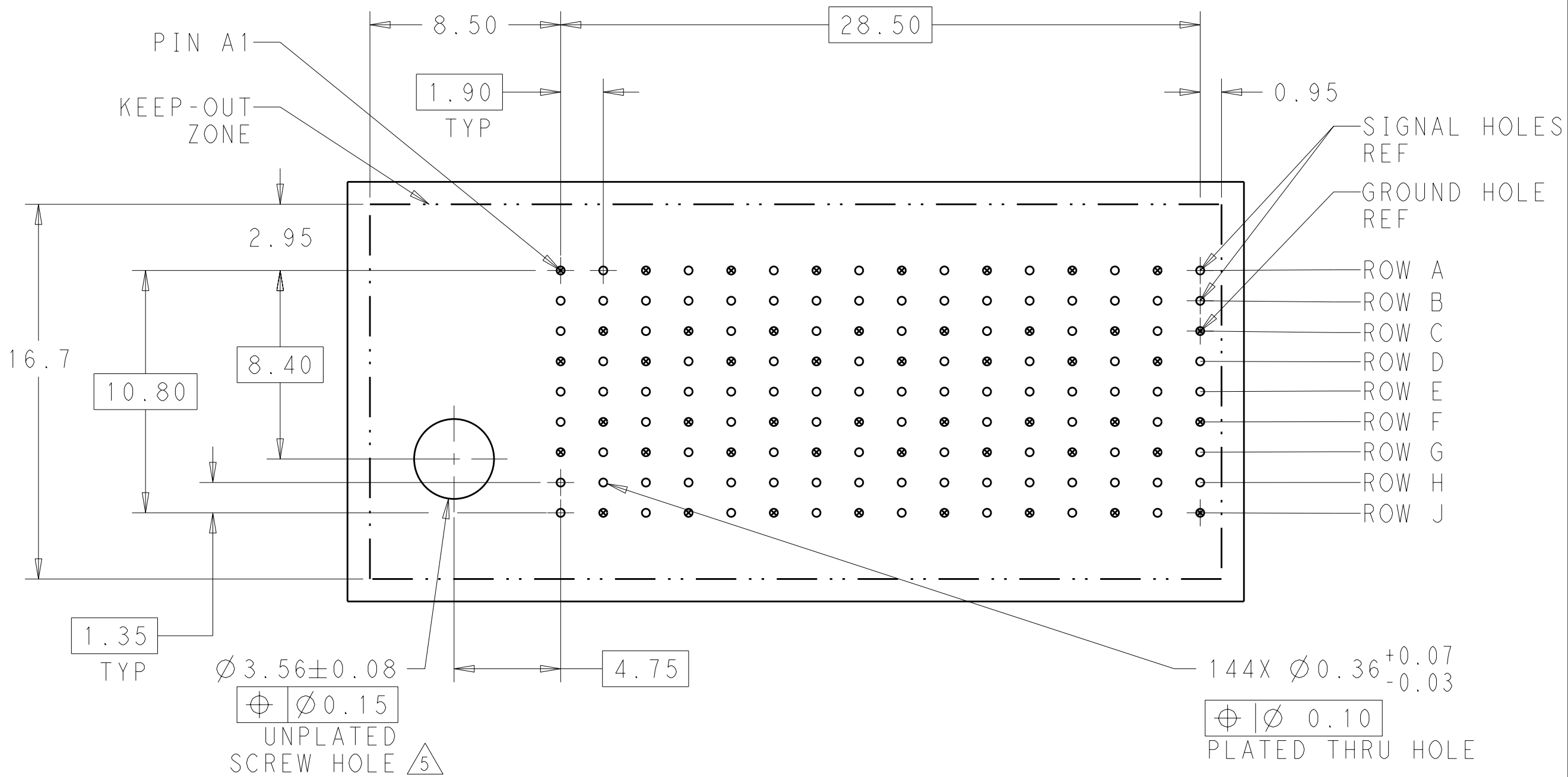
LEFT GUIDED BACKPLANE HOLE PATTERN (CONNECTOR SIDE)
