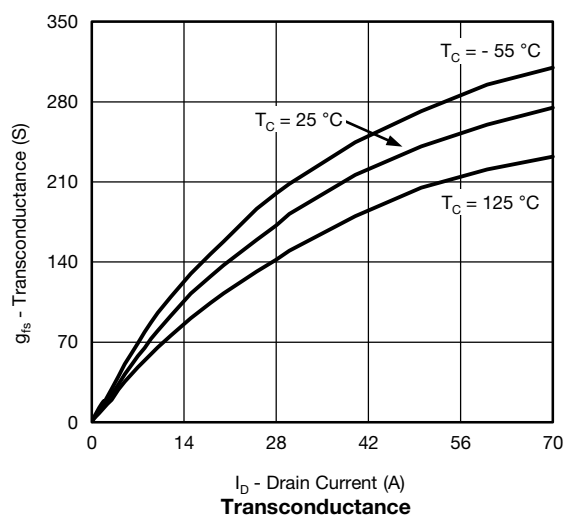
Transconductance
