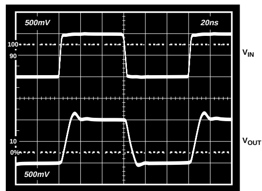
Figure 26. Small Signal Pulse Response, Gain = +1, ( R_F = 750\ \Omega , R_L = 150\ \Omega , V_S = \pm 5\ \text{V} )
