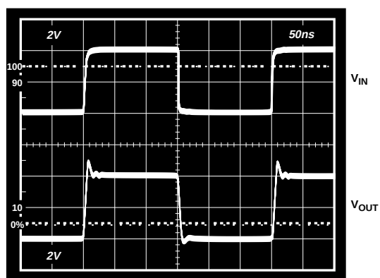
Figure 23. Large Signal Pulse Response, Gain = +1, ( R_F = 750\ \Omega , R_L = 150\ \Omega , V_S = \pm 5\ \text{V} )
