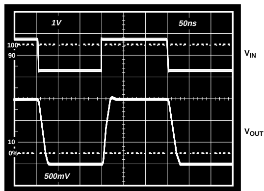
Figure 55. Pulse Response of the Circuit of Figure 53 with V_S = 5V
