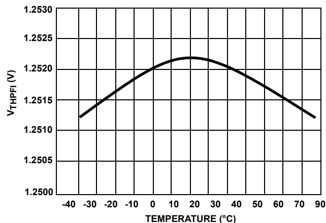
FIGURE 9. V_{THPFI} vs TEMPERATURE
