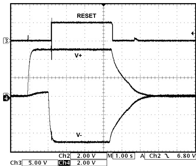
FIGURE 16. ±5V MONITORING
