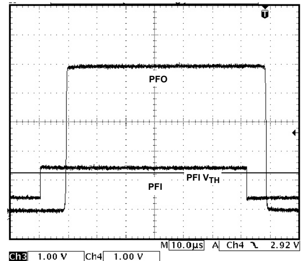
FIGURE 13. 5V PFI TO PFO RESPONSE
