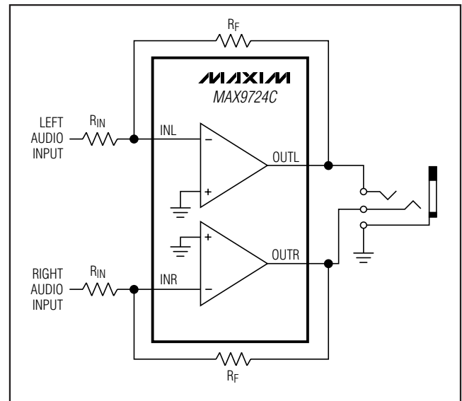
Figure 3. Gain Setting for the MAX9724C
