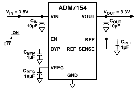
Figure 1. Regulated 3.3 V Output from 3.8 V Input
