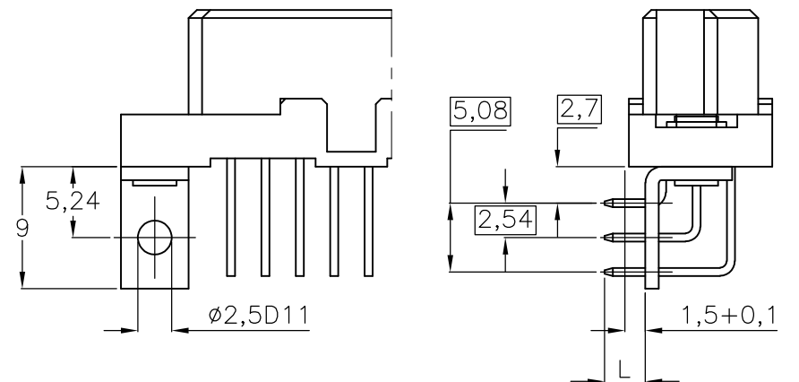
FEMALE CONNECTOR WITH RIGHT ANGLE SOLDER LEADS WITH MOUNTING BRACKET
