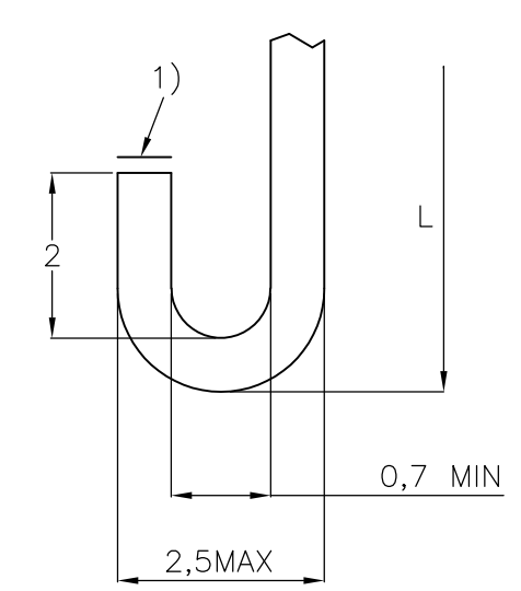
SOLDER HOOKS
