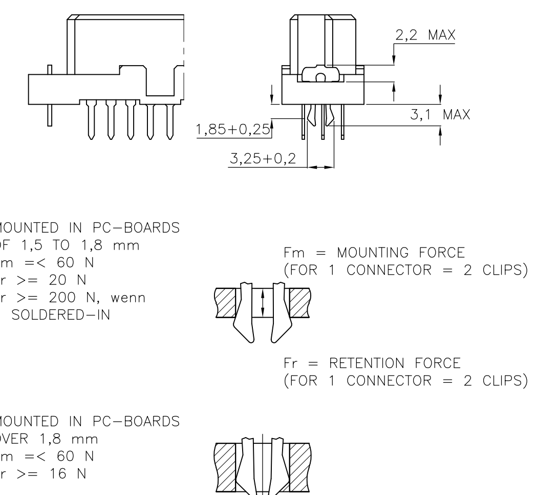
Female connector with board locks
