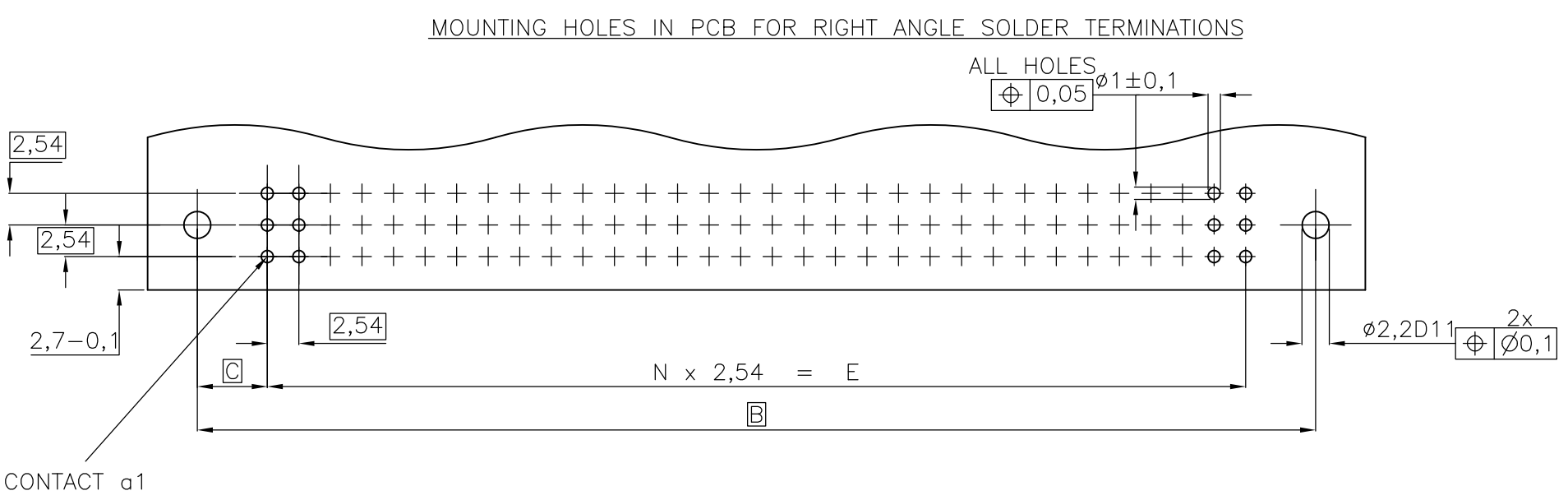
FEMALE CONNECTOR WITH RIGHT ANGLE SOLDER LEADS WITH MOUNTING BRACKET
