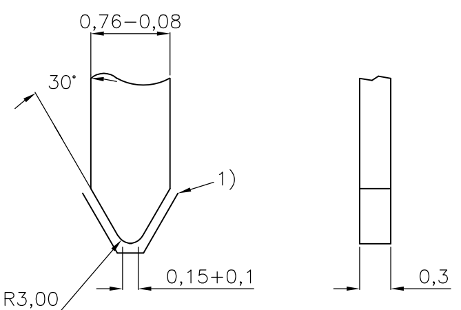
WIRE WRAP TERMINATIONS AND SOLDER TERMINATION
