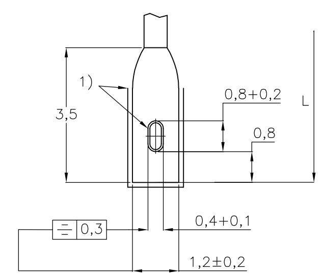
SOLDER LUGS
