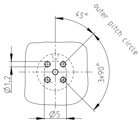
PCB-Layout (advice)
