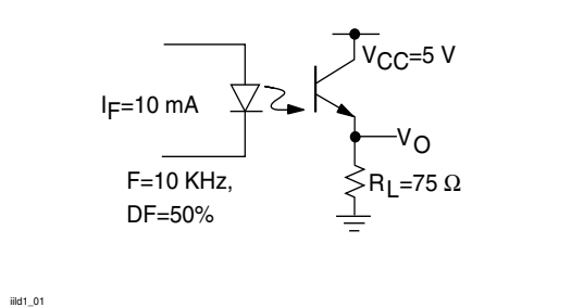
Figure 1. Non-saturated Switching Schematic
