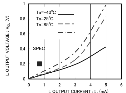
Fig.5 'L' output voltage V_{OL1} - I_{OL} ( V_{CC}=1.7\text{V} )
