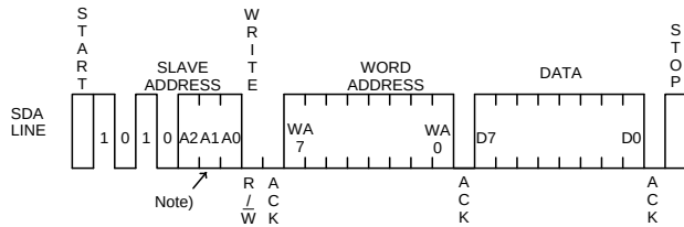
Fig.38 Byte write cycle (BR24T01/02/04/08/16-W)
