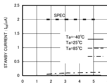
Fig.14 Standby operation I_{bb} (f scl =400kHz BR24T01/02/04/08/16/32/64/128/256-W)
