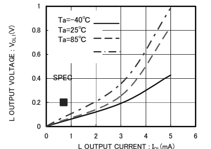
Fig.5 'L' output voltage V_{OL1}-I_{OL} ( V_{CC}=1.7V )
