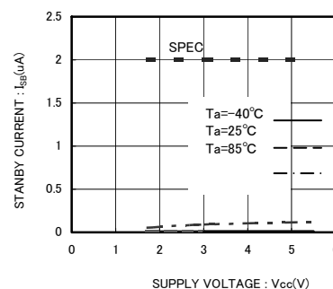
Fig.14 Standby operation I_{SB} (fsc1=400kHz BR24T01/02/04/08/16/32/64/128/256-W)
