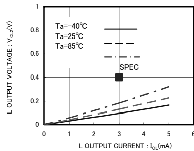
Fig.6 'L' output voltage V_{OL2} \sim V_{OL}(V_{CC}=2.5V)
