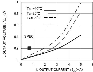
Fig.5 'L' output voltage V_{OL1} \sim V_{OL}(V_{CC}=1.7V)
