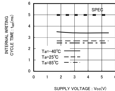
Fig.29 Internal writing cycle time t_{WR}
