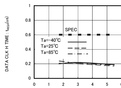
Fig.17 Data clock High Period t_{HIGH}
