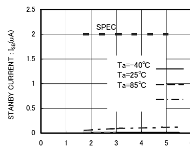
Fig.14 Standby operation I_{bb} (f sc =400kHz BR24T01/02/04/08/16/32/64/128/256-W)
