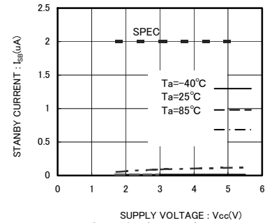
Fig.14 Standby operation I_{bb} (f scl =400kHz BR24T01/02/04/08/16/32/64/128/256-W)
