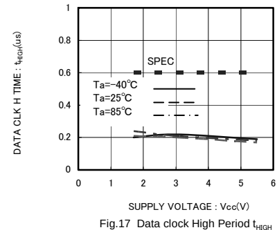
Fig.17 Data clock High Period t_{HIGH}
