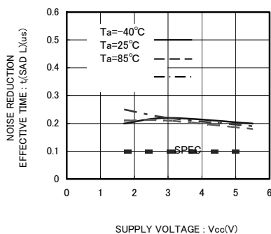
Fig.33 Noise reduction effective time t_t(\text{SDA L})
