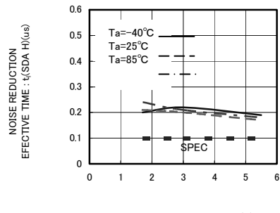
Fig.32 Noise reduction effective time t_t(\text{SDA H})
