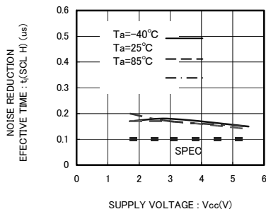
Fig.30 Noise reduction effective time t_t(\text{SCL H})
