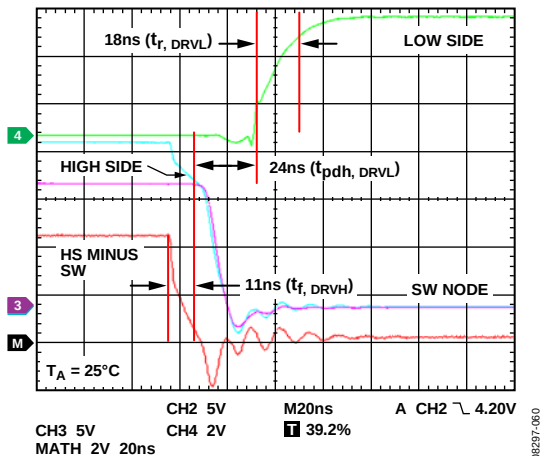
Figure 60. Upper Side Driver Falling and Lower Side Rising Edge Waveforms ( C_{\text{GATE}} = 4.3 \text{ nF} (Upper/Lower Side MOSFET), Q_{\text{TOTAL}} = 27 \text{ nC} ( V_{GS} = 4.4 \text{ V} (Q1), V_{GS} = 5 \text{ V} (Q3))
