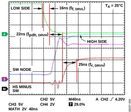
Figure 59. Upper Side Driver Rising and Lower Side Falling Edge Waveforms ( C_{\text{GATE}} = 4.3 \text{ nF} (Upper/Lower Side MOSFET), Q_{\text{TOTAL}} = 27 \text{ nC} ( V_{GS} = 4.4 \text{ V} (Q1), V_{GS} = 5 \text{ V} (Q3))
