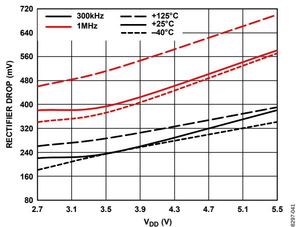
Figure 41. Internal Boost Rectifier Drop vs. V_{DD}
