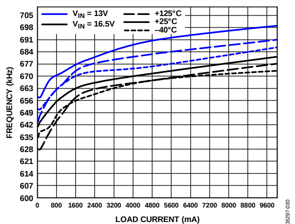
Figure 30. Frequency vs. Load Current, 600 kHz, V_{OUT} = 5\text{ V}
