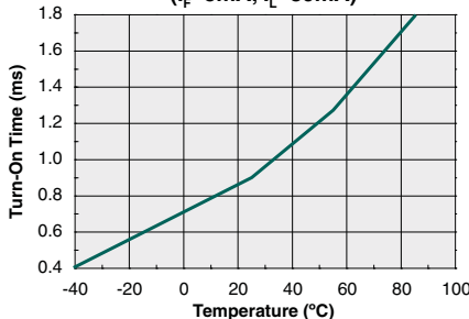
Typical Turn-On Time vs. Temperature ( I_F=5\text{mA} , I_L=80\text{mA} )
