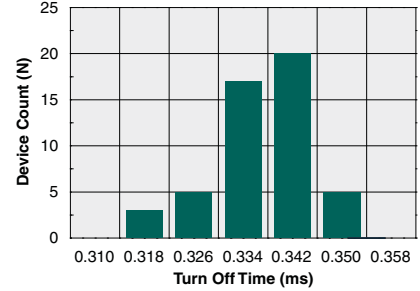
Turn-Off Time (N=50, I_F=5\text{mA} , I_L=120\text{mA} )
