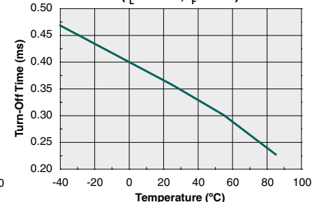
Typical Turn-Off Time vs. Temperature ( I_L=80\text{mA} , I_F=5\text{mA} )
