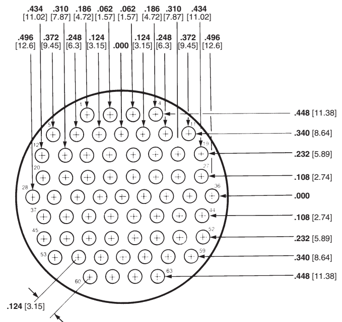
Arrangement 23-63 Max. Wire Ins. Dia. = .068 [1.73]
