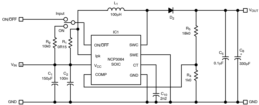
Figure 20. Typical Boost Application Schematic
