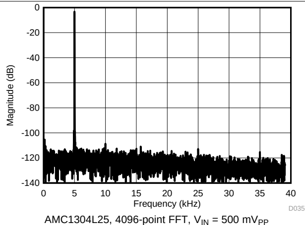
Figure 37. Frequency Spectrum with 5-kHz Input Signal
