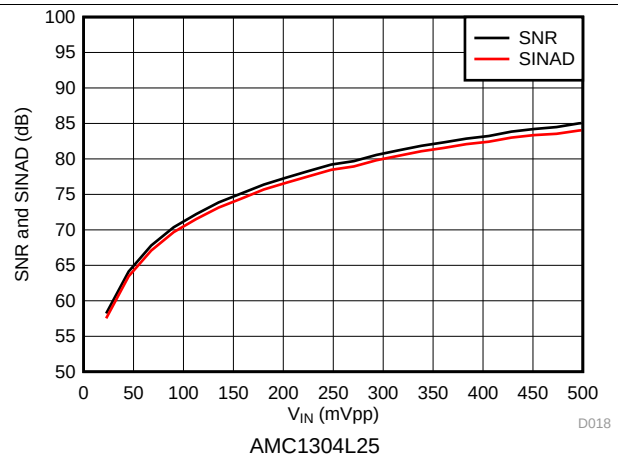
Figure 20. SNR and SINAD vs Input Signal Amplitude
