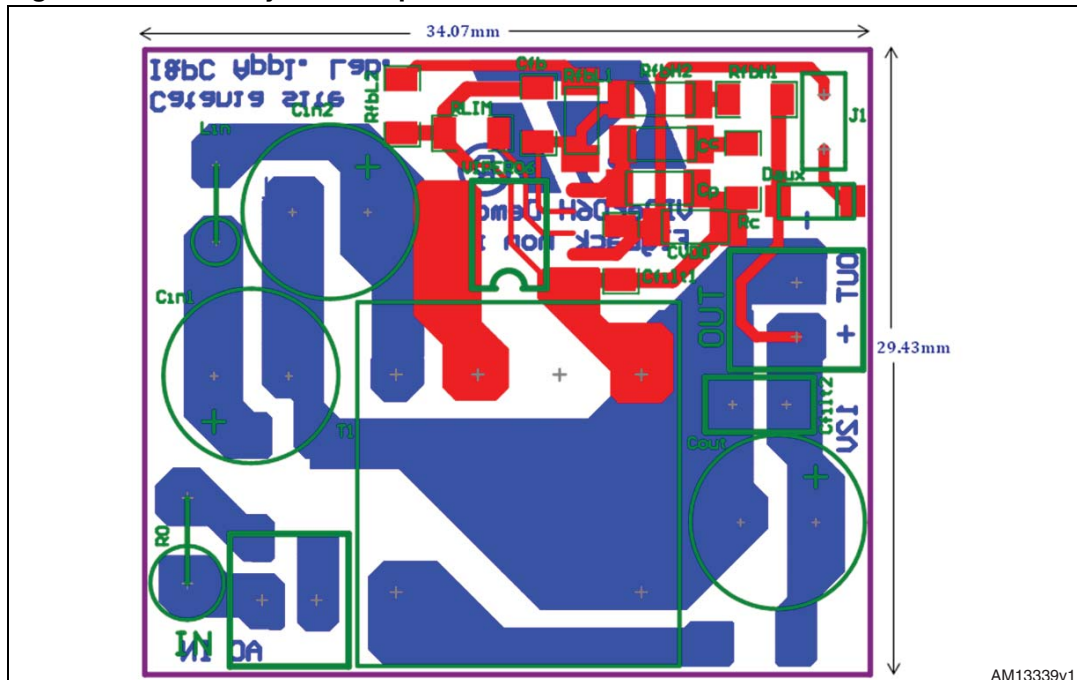
Figure 18. Board layout - complete
