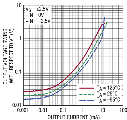
Output Voltage Swing vs Load Current (Sink)
