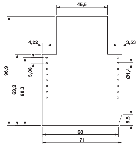
Dimensional drawing
