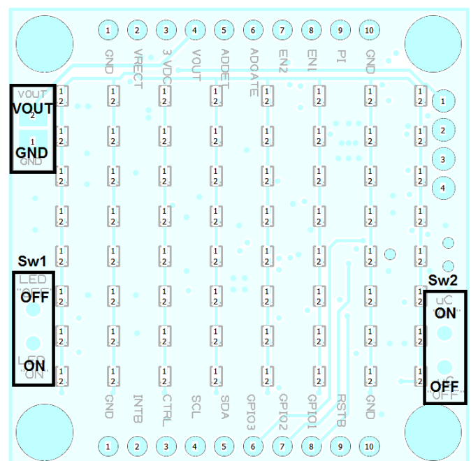
Figure 7: LED Module, top view
