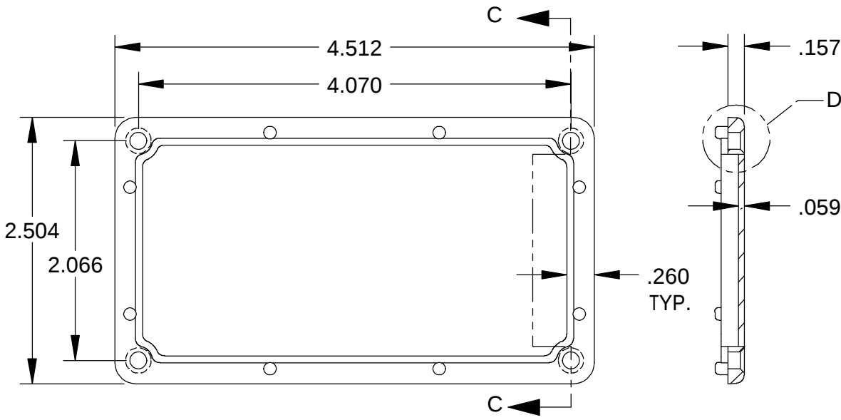
SECTION C-C
