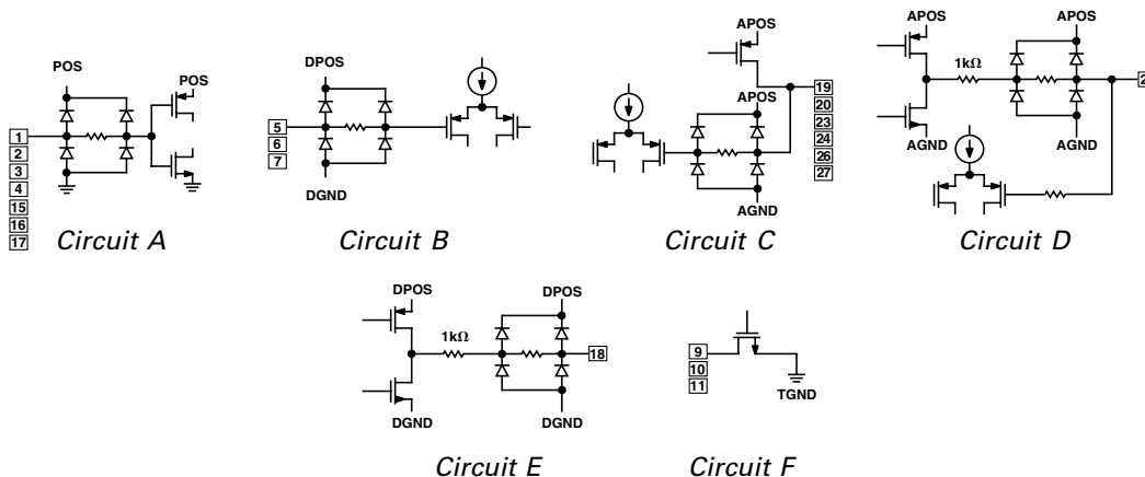
Figure 1. Equivalent Circuits
