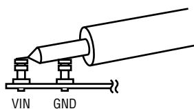
Figure 2. Measuring Input or Output Ripple
