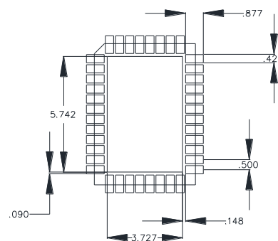
SOLDER MASK
