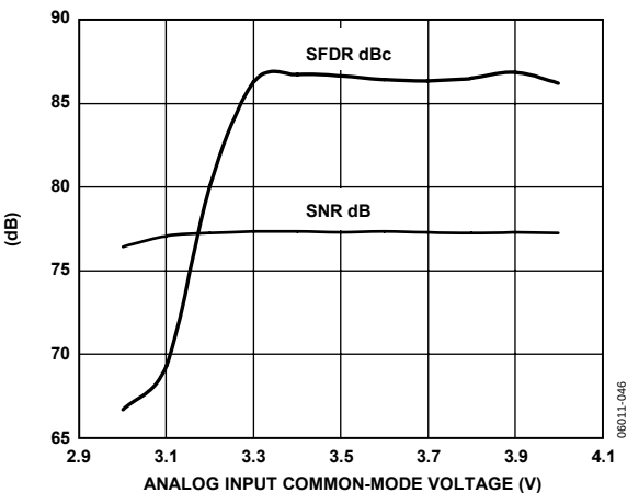
Figure 27. 130 MSPS, SNR/SFDR vs. Analog Input Common Mode
