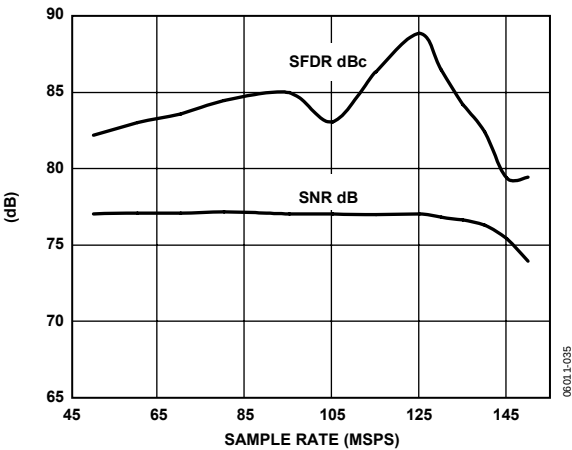
Figure 28. Single-Tone SNR/SFDR vs. Sample Rate 170.3 MHz
