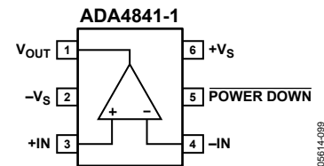
Figure 2. 6-Lead SOT-23 (R)
