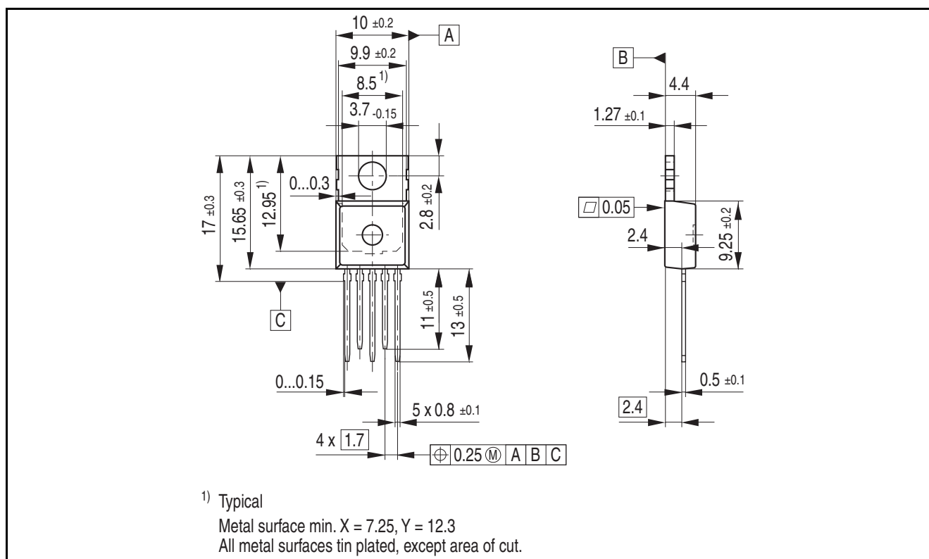
Figure 2 PG-TO220-5-12
