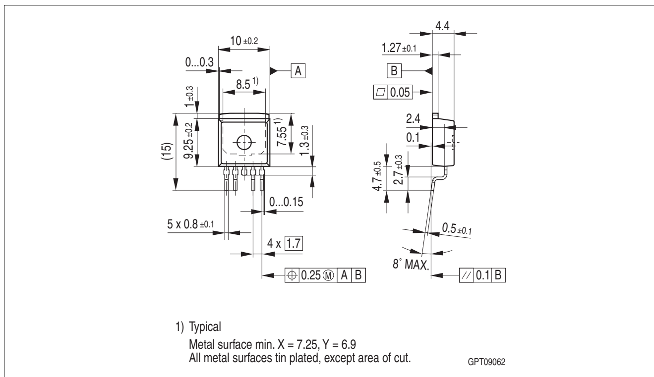
Figure 1 PG-TO263-5-2
