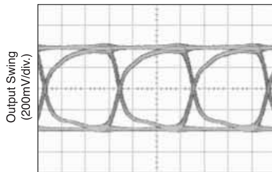
3.2Gbps Output
