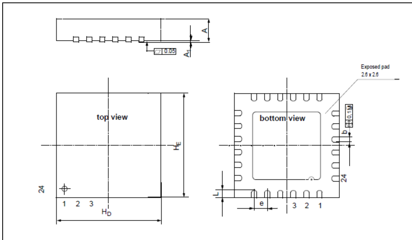
Figure 5.1 24-pin QFN Package Drawing
