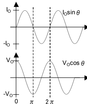
Fig.1.7 the Output current and Output Voltage with inductance load
